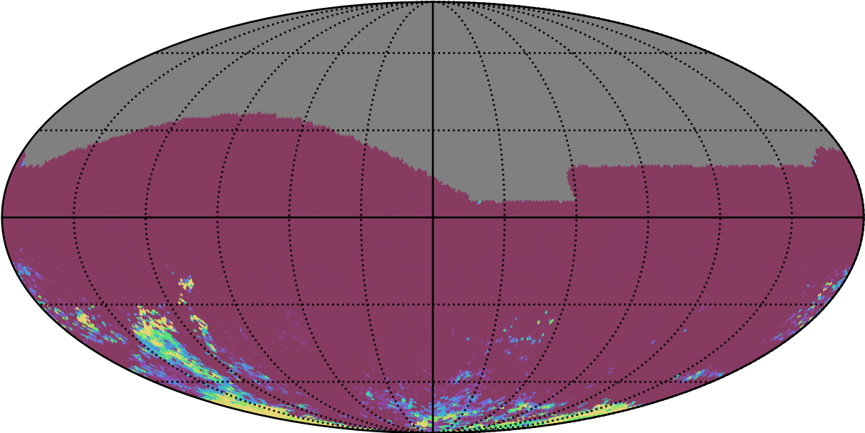
too_elab_r16_d3_griz_v3.4_10yrs All sky gr bands: 75th Percentile Intranight Timespan
