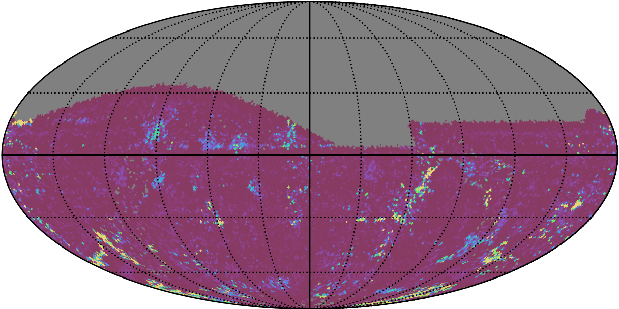
too_elab_r16_d3_griz_v3.4_10yrs All sky g band: 75th Percentile Intranight Timespan
