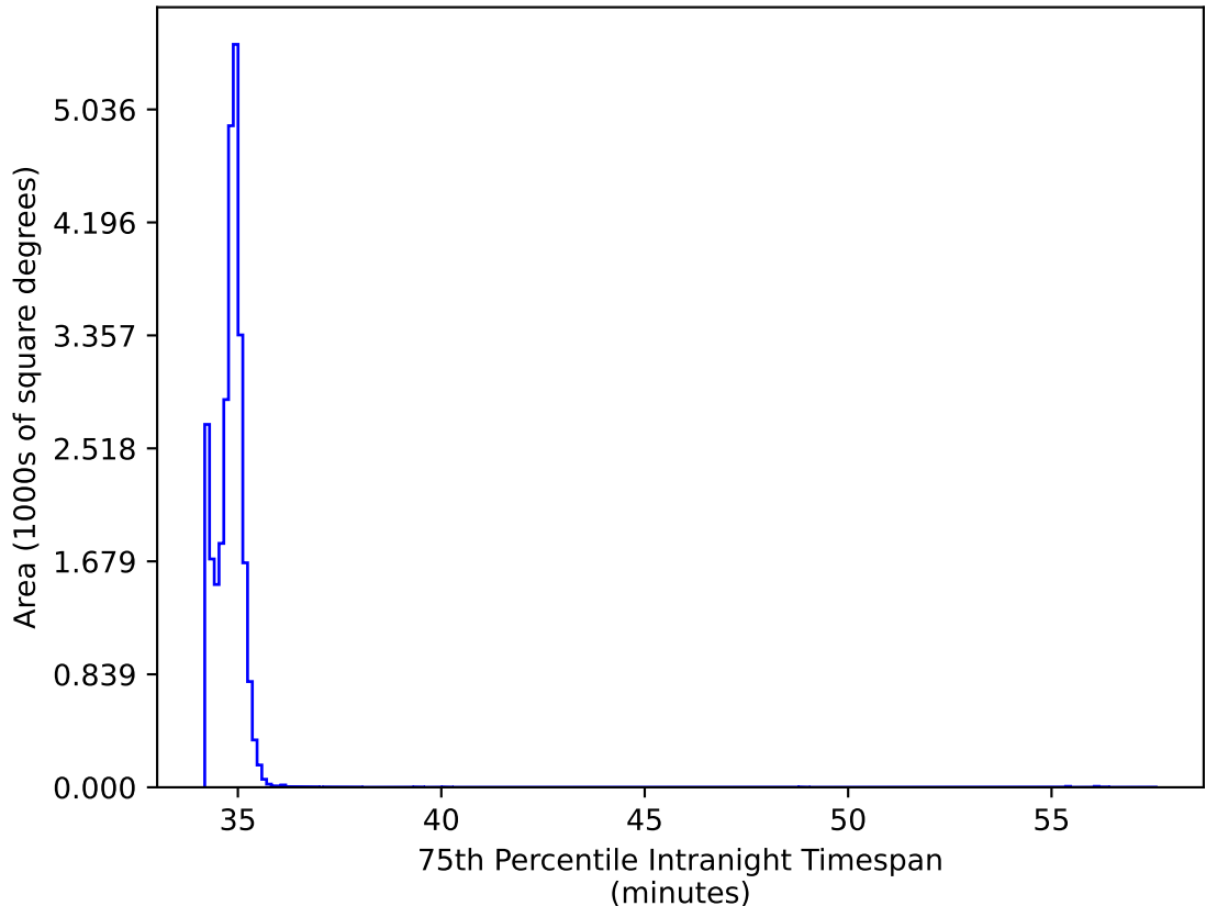
too_elab_r16_d3_griz_v3.4_10yrs All sky: 75th Percentile Intranight Timespan
