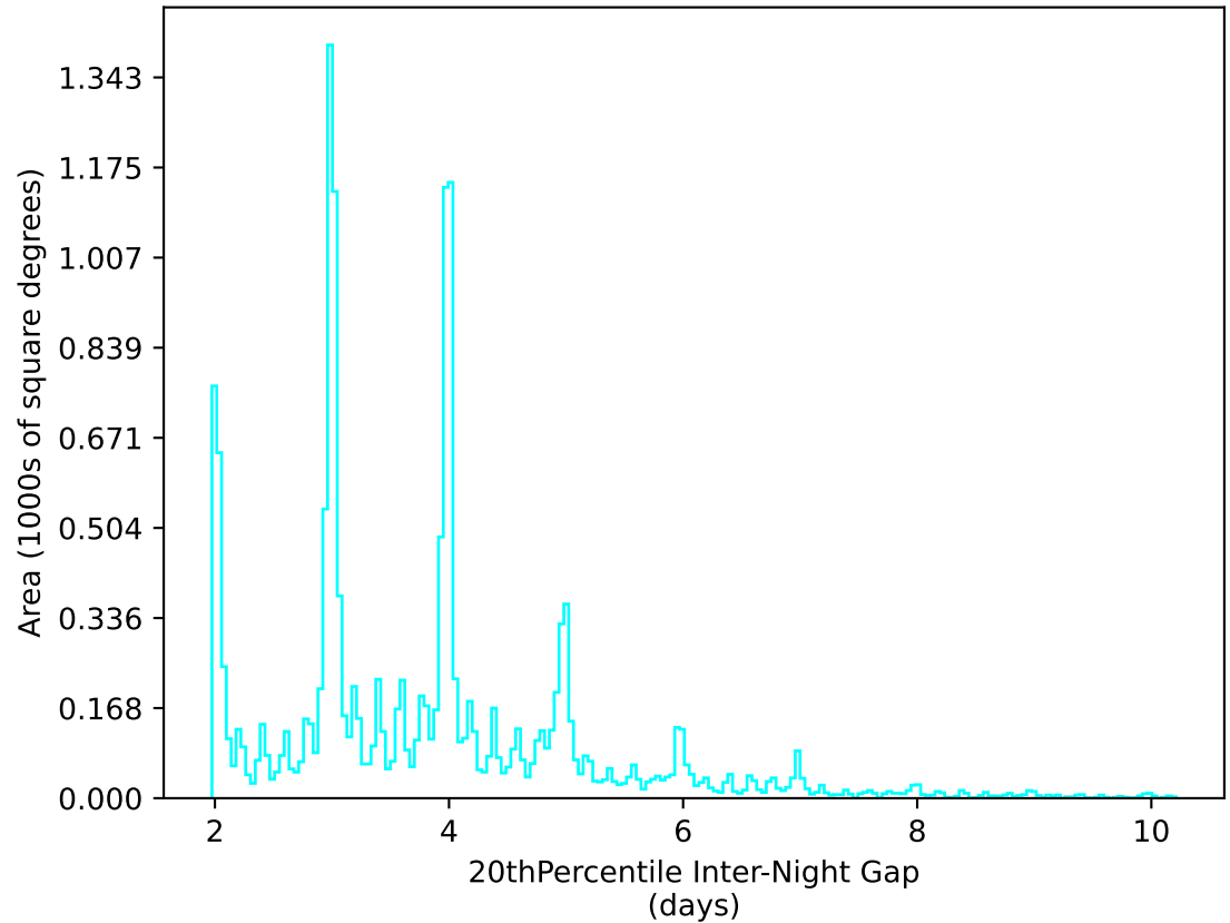
too_elab_r16_d3_griz_v3.4_10yrs WFD u band: 20thPercentile Inter-Night Gap
