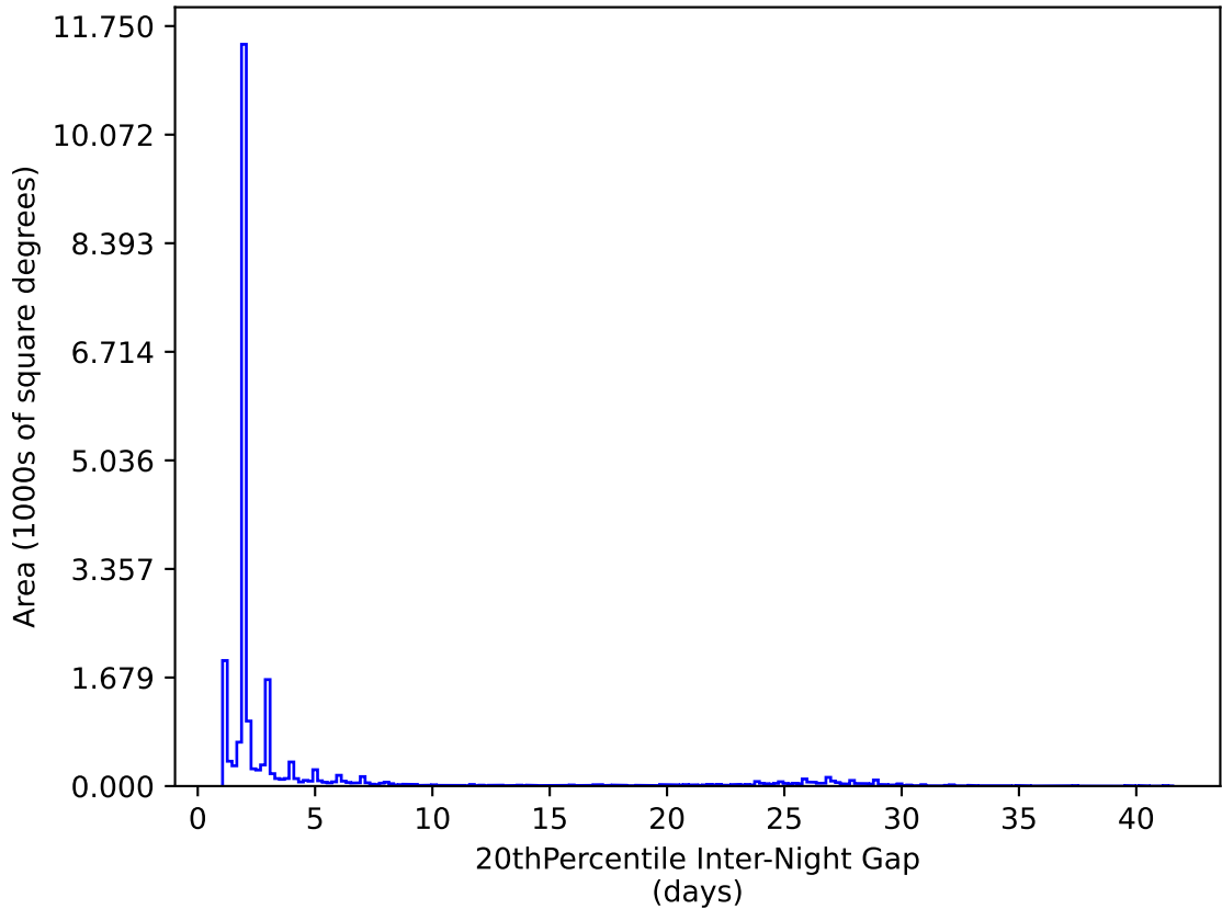
too_elab_r16_d3_griz_v3.4_10yrs All sky y band: 20thPercentile Inter-Night Gap
