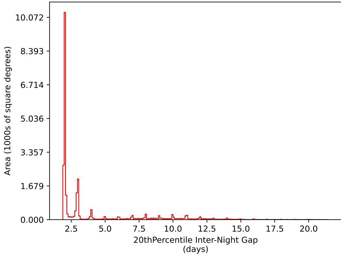
too_elab_r16_d3_griz_v3.4_10yrs All sky i band: 20thPercentile Inter-Night Gap
