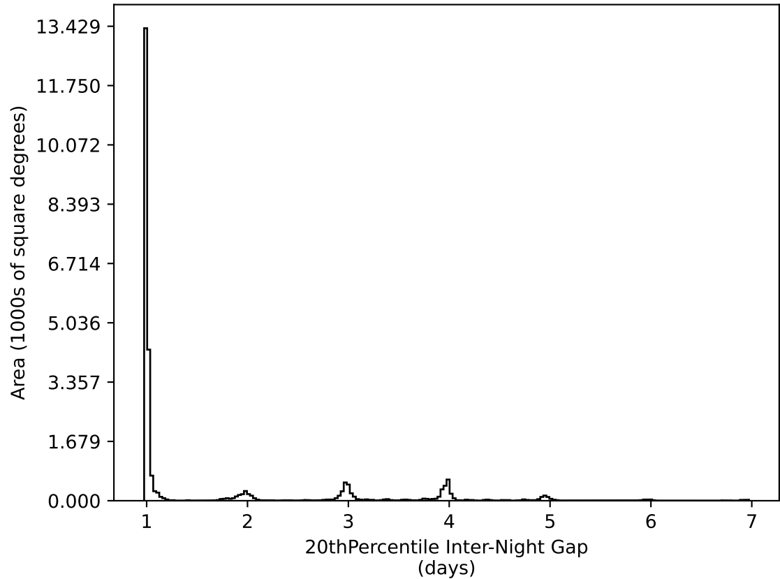
too_elab_r16_d3_griz_v3.4_10yrs All sky all bands: 20thPercentile Inter-Night Gap
