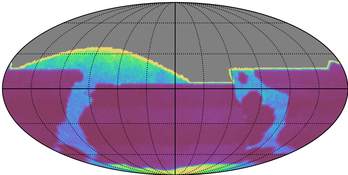
too_elab_r16_d3_griz_v3.4_10yrs : properMotion
