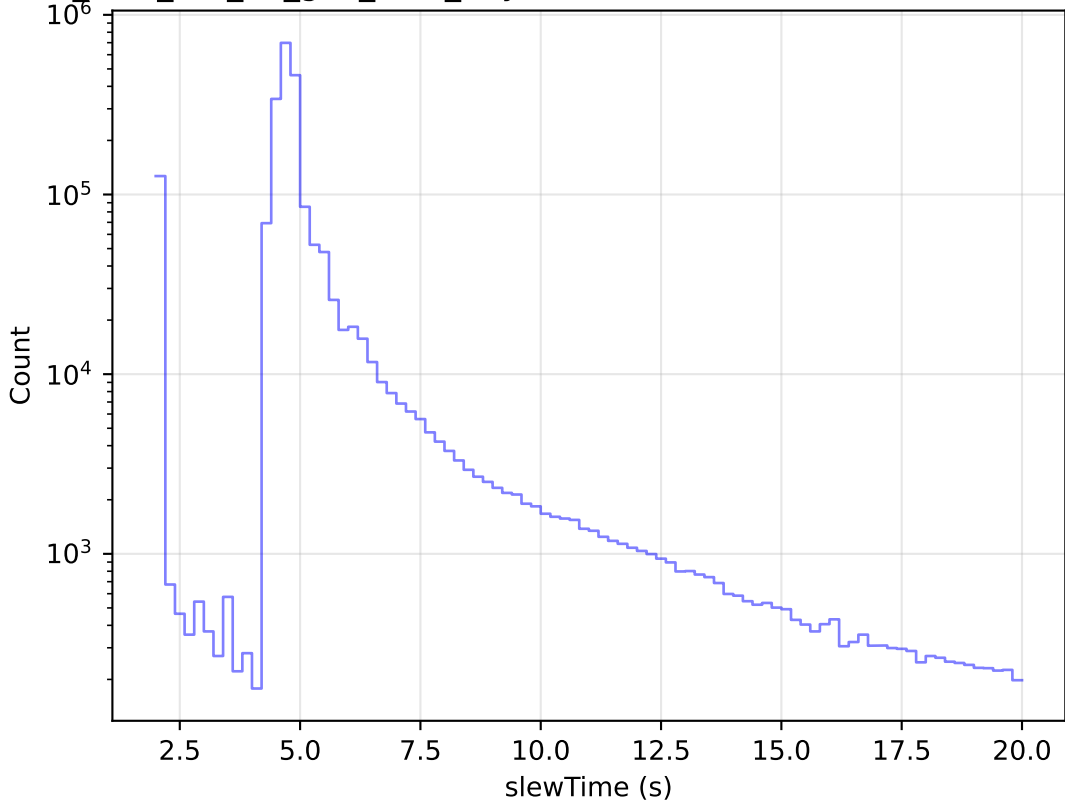
too_elab_r16_d3_griz_v3.4_10yrs All visits: Zoom Slew Time Histogram
