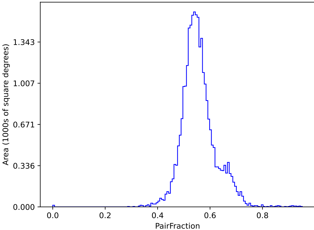
too_elab_r16_d3_griz_v3.4_10yrs (g or r or i): PairFraction
