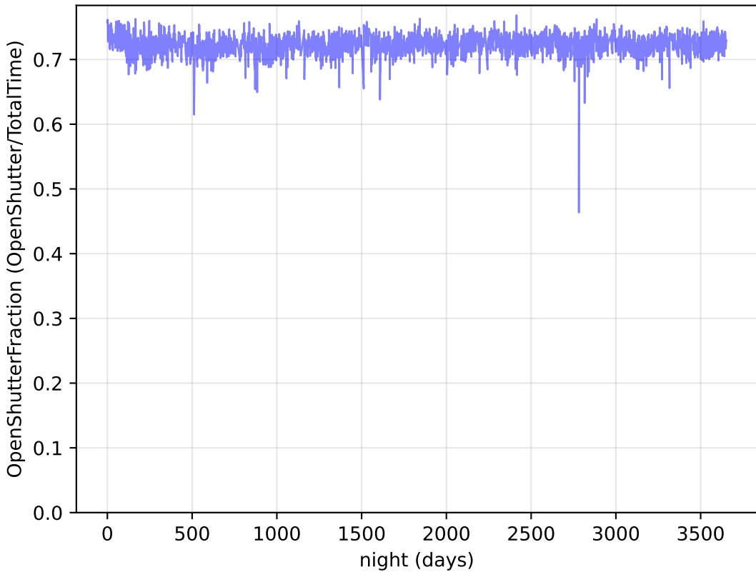
too_elab_r16_d3_griz_v3.4_10yrs : OpenShutterFraction
