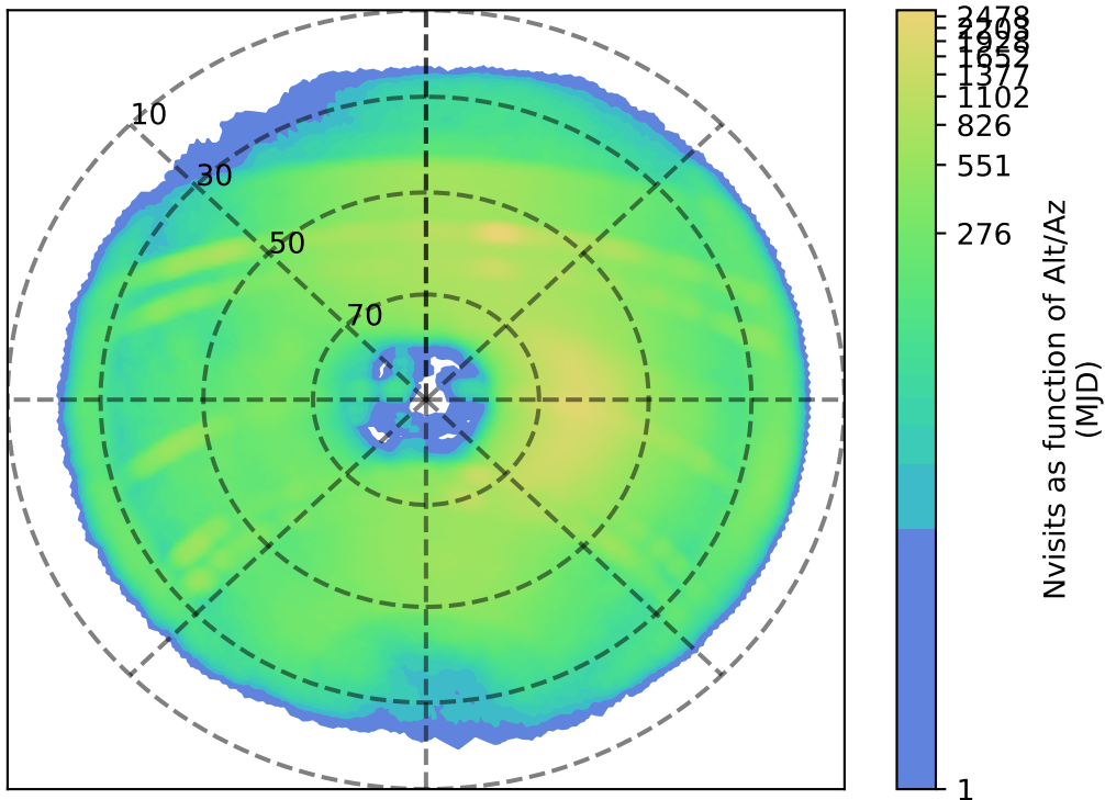
too_elab_r16_d3_griz_v3.4_10yrs z: Nvisits as function of Alt/Az
