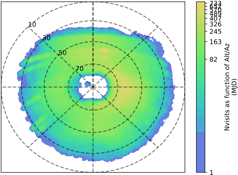
too_elab_r16_d3_griz_v3.4_10yrs u: Nvisits as function of Alt/Az
