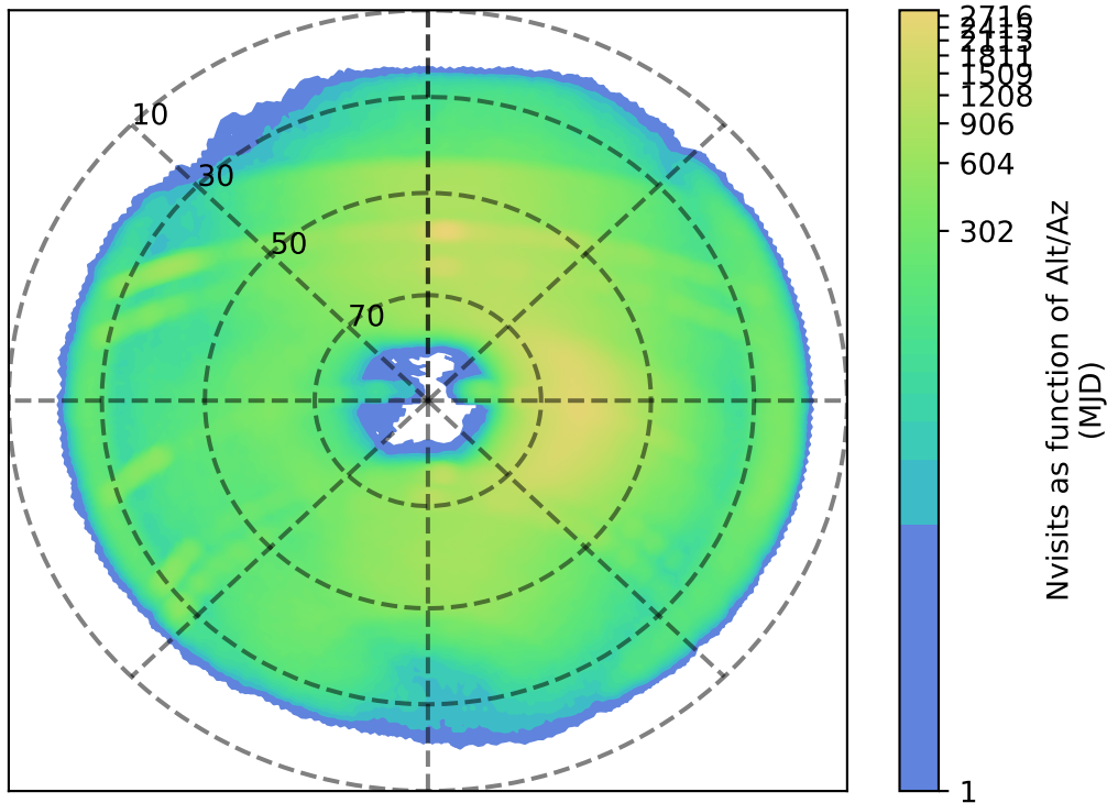
too_elab_r16_d3_griz_v3.4_10yrs i: Nvisits as function of Alt/Az
