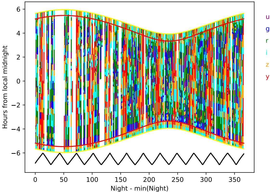
too_elab_r16_d3_griz_v3.4_10yrs year 8-9: Hourglass
