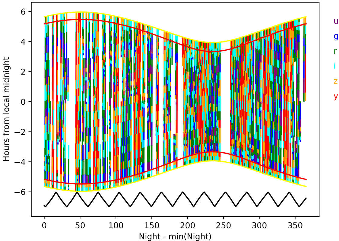
too_elab_r16_d3_griz_v3.4_10yrs year 5-6: Hourglass
