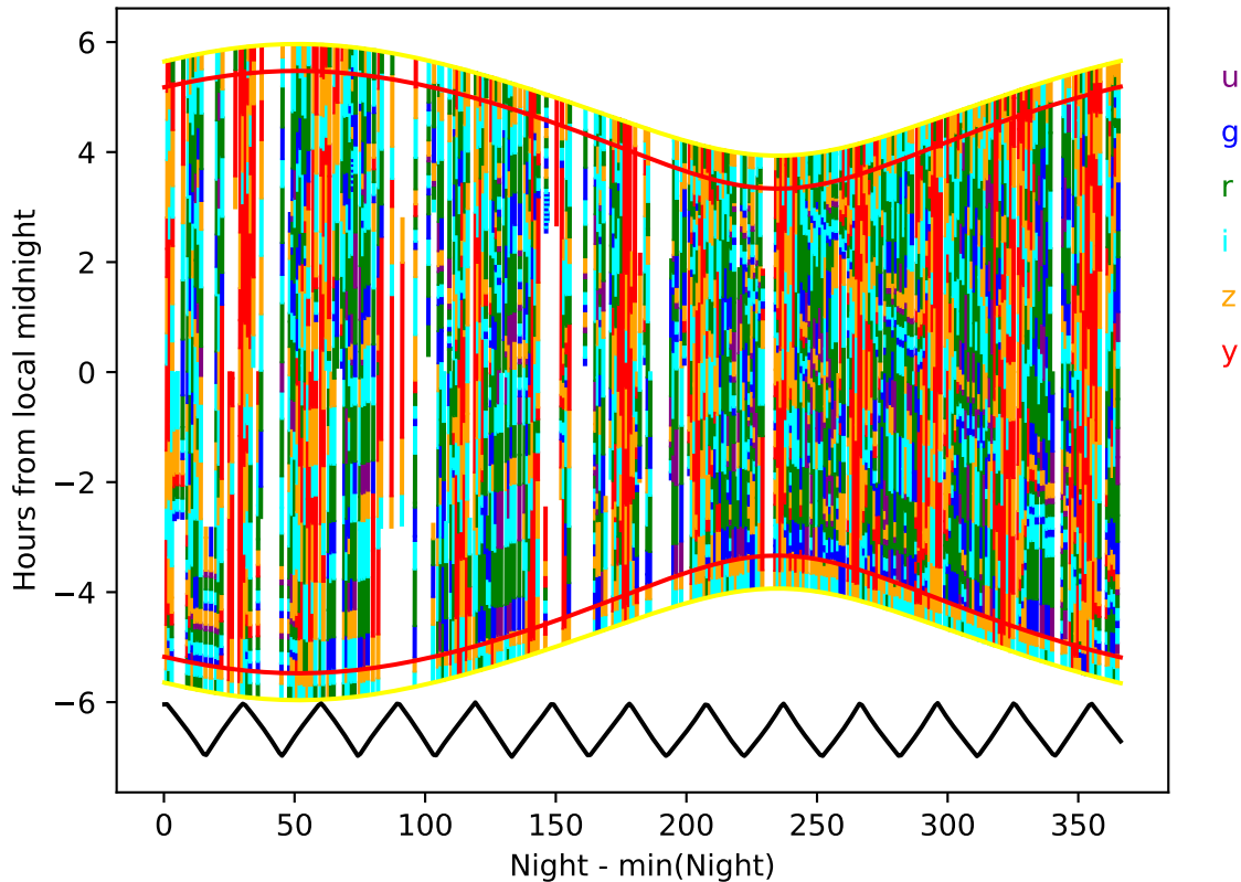
too_elab_r16_d3_griz_v3.4_10yrs year 1-2: Hourglass
