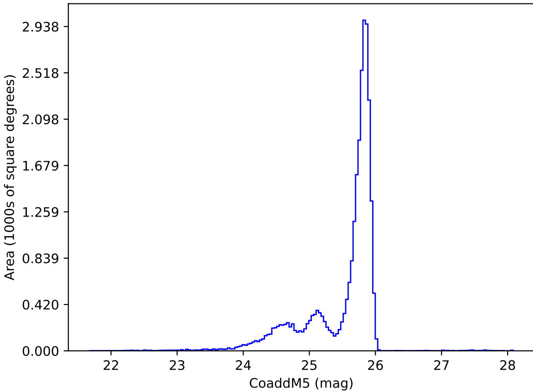
too_elab_r16_d3_griz_v3.4_10yrs z: CoaddM5
