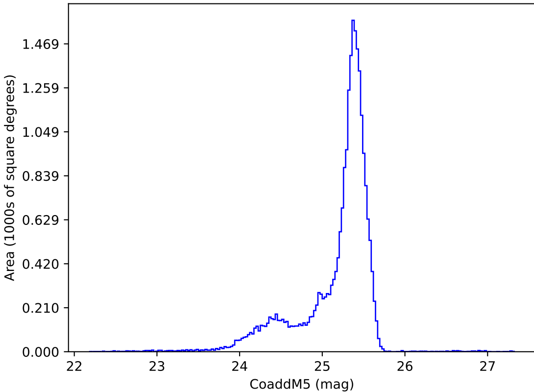
too_elab_r16_d3_griz_v3.4_10yrs u: CoaddM5
