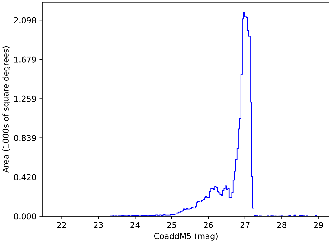
too_elab_r16_d3_griz_v3.4_10yrs r: CoaddM5
