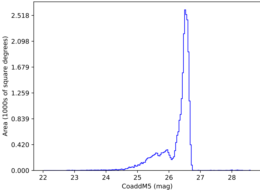
too_elab_r16_d3_griz_v3.4_10yrs i: CoaddM5
