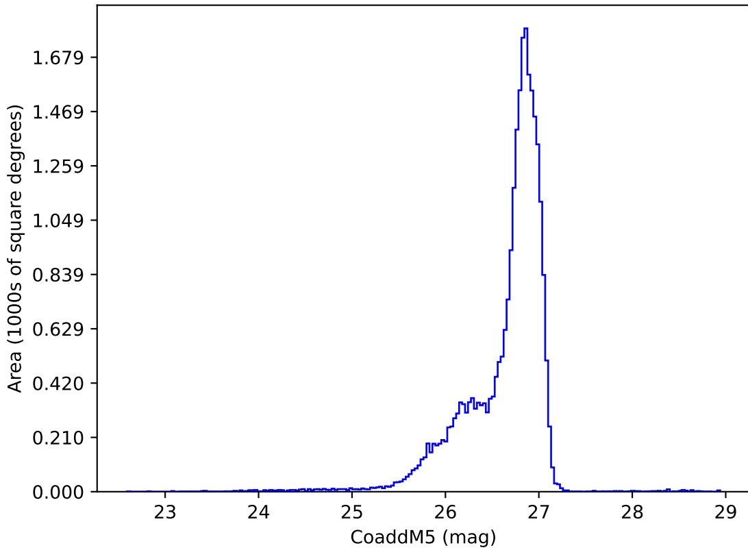
too_elab_r16_d3_griz_v3.4_10yrs g: CoaddM5
