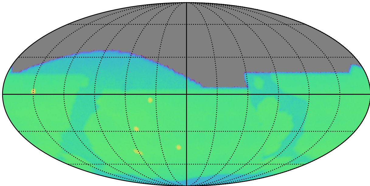
too_elab_r16_d3_griz_v3.4_10yrs : CoaddM5
