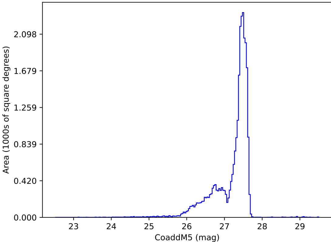
too_elab_r16_d3_griz_v3.4_10yrs : CoaddM5
