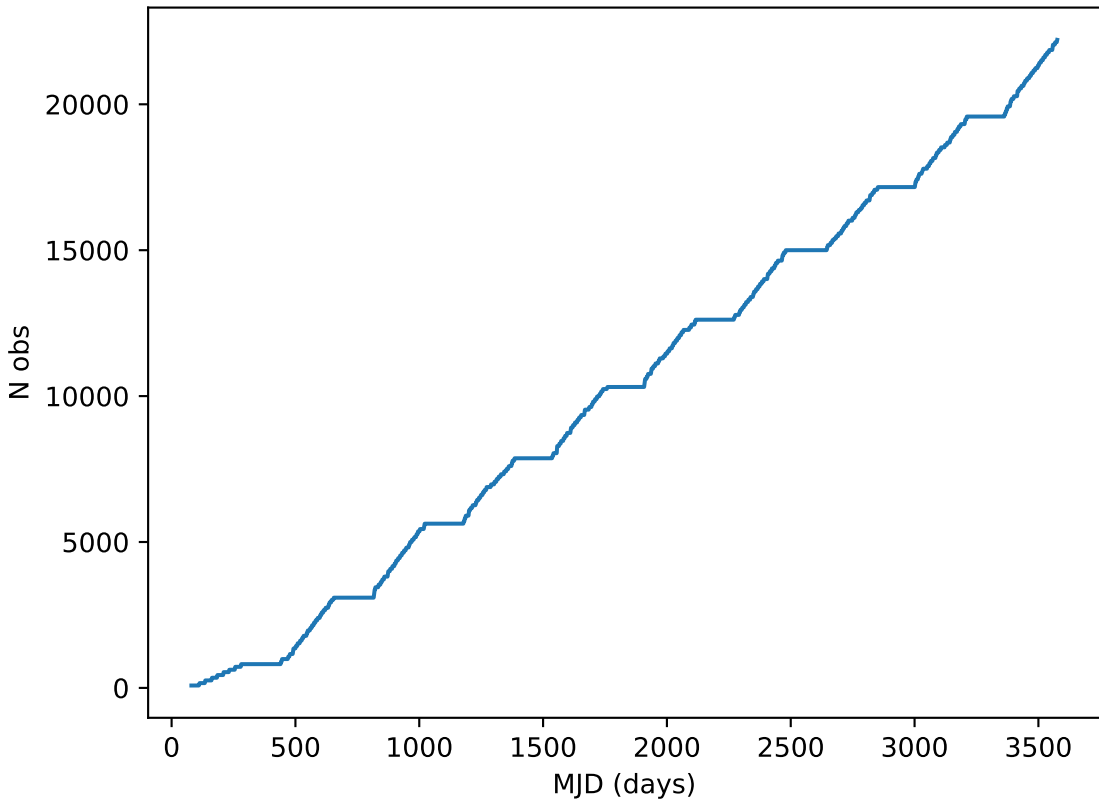
too_elab_r16_d3_griz_v3.4_10yrs all bands: DD:XMM_LSS Cumulative NVisits
