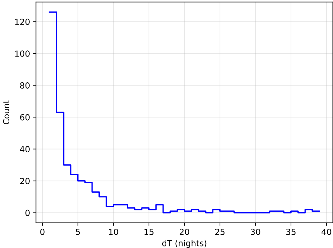
too_elab_r16_d3_griz_v3.4_10yrs all bands: DD:WFD Delta Nights Histogram
