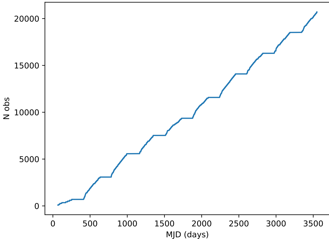
too_elab_r16_d3_griz_v3.4_10yrs all bands: DD:ELAISS1 Cumulative NVisits
