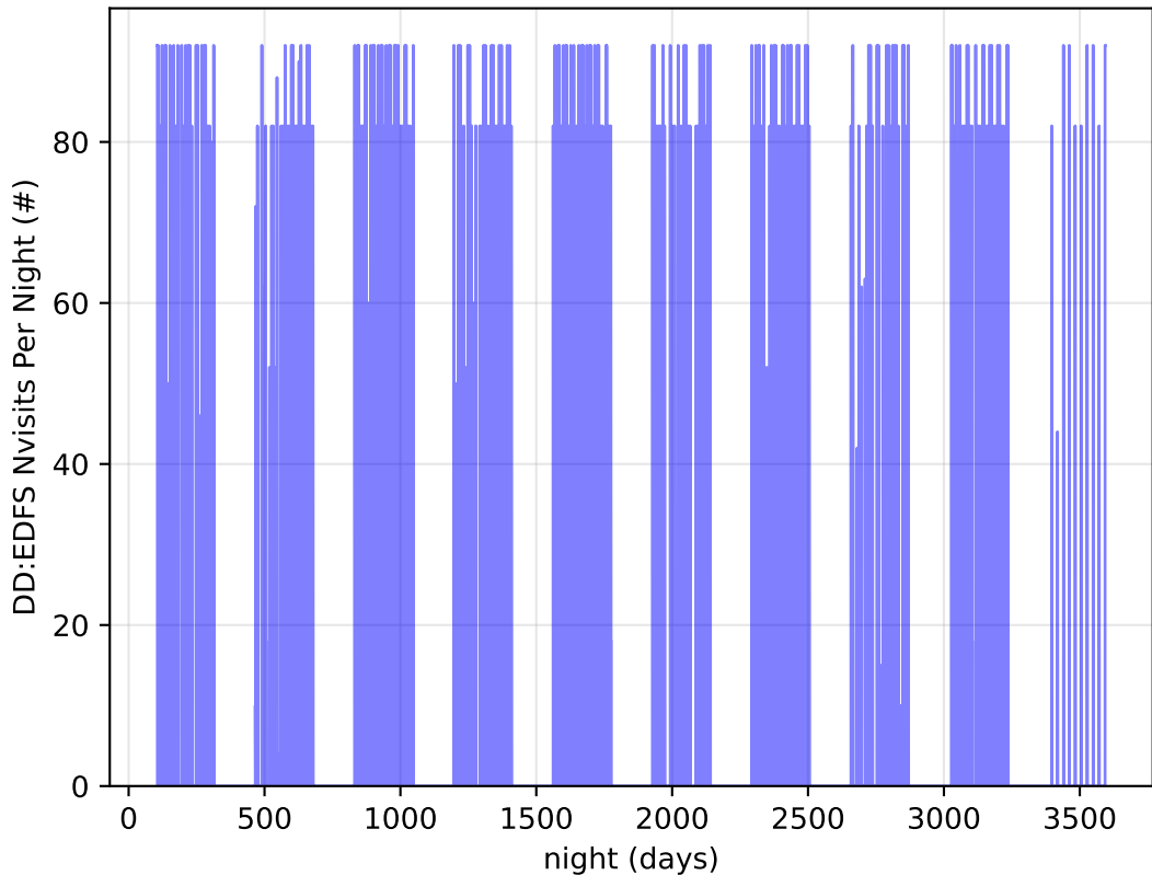
too_elab_r16_d3_griz_v3.4_10yrs all bands: DD:EDFS Nvisits Per Night
