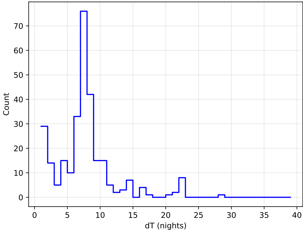
too_elab_r16_d3_griz_v3.4_10yrs all bands: DD:EDFS Delta Nights Histogram
