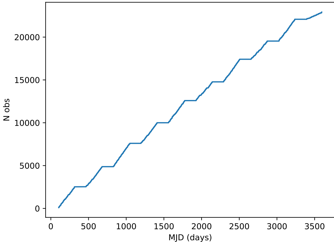
too_elab_r16_d3_griz_v3.4_10yrs all bands: DD:EDFS Cumulative NVisits
