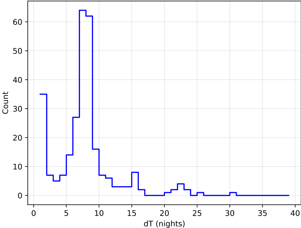
too_elab_r16_d3_griz_v3.4_10yrs all bands: DD:ECDFS Delta Nights Histogram
