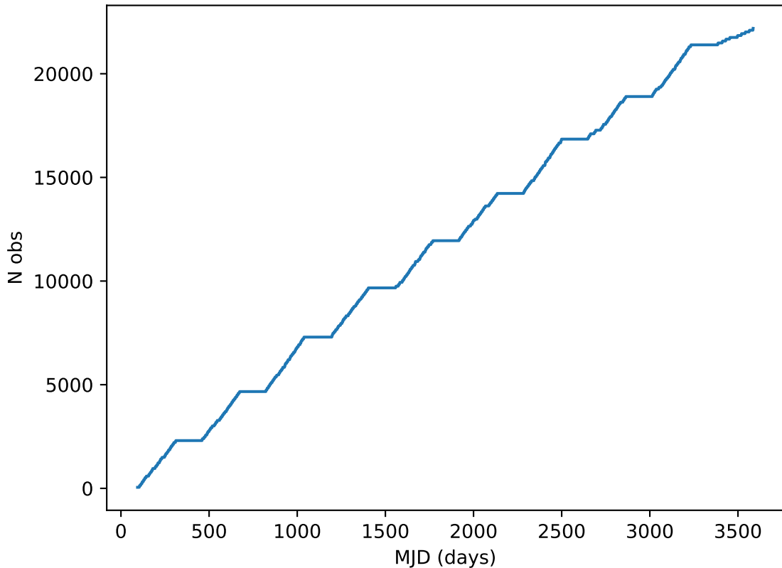
too_elab_r16_d3_griz_v3.4_10yrs all bands: DD:ECDFS Cumulative NVisits
