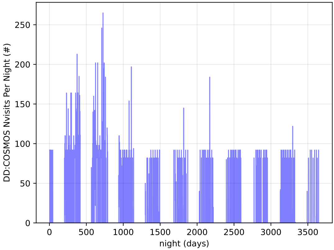
too_elab_r16_d3_griz_v3.4_10yrs all bands: DD: COSMOS Nvisits Per Night
