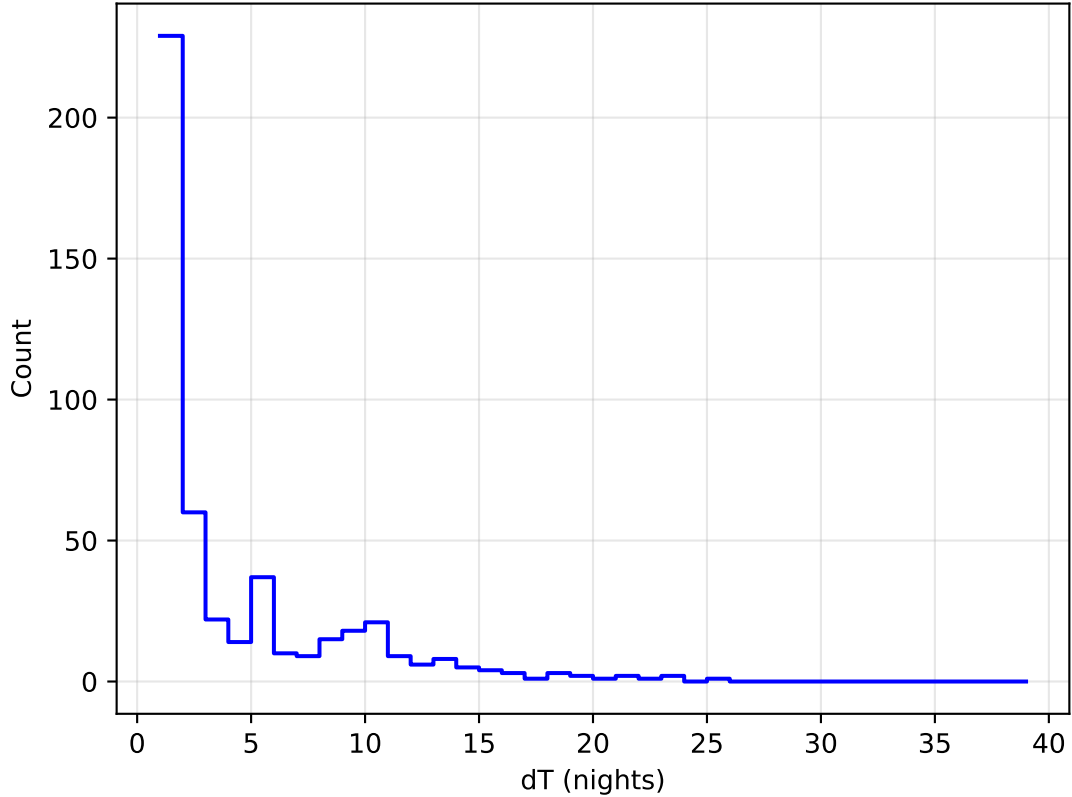
too_elab_r16_d3_griz_v3.4_10yrs all bands: DD: COSMOS Delta Nights Histogram
