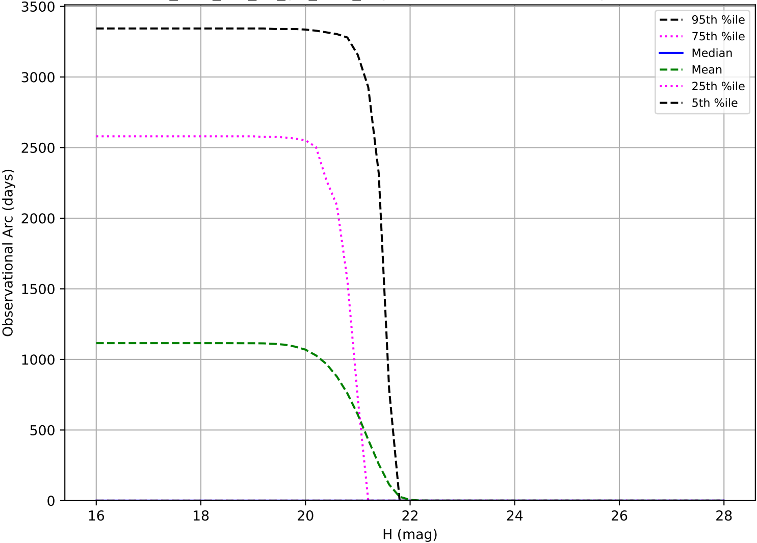
too_elab_r16_d3_giz_v3.4_10yrs: Observational Arc Length Vatira
