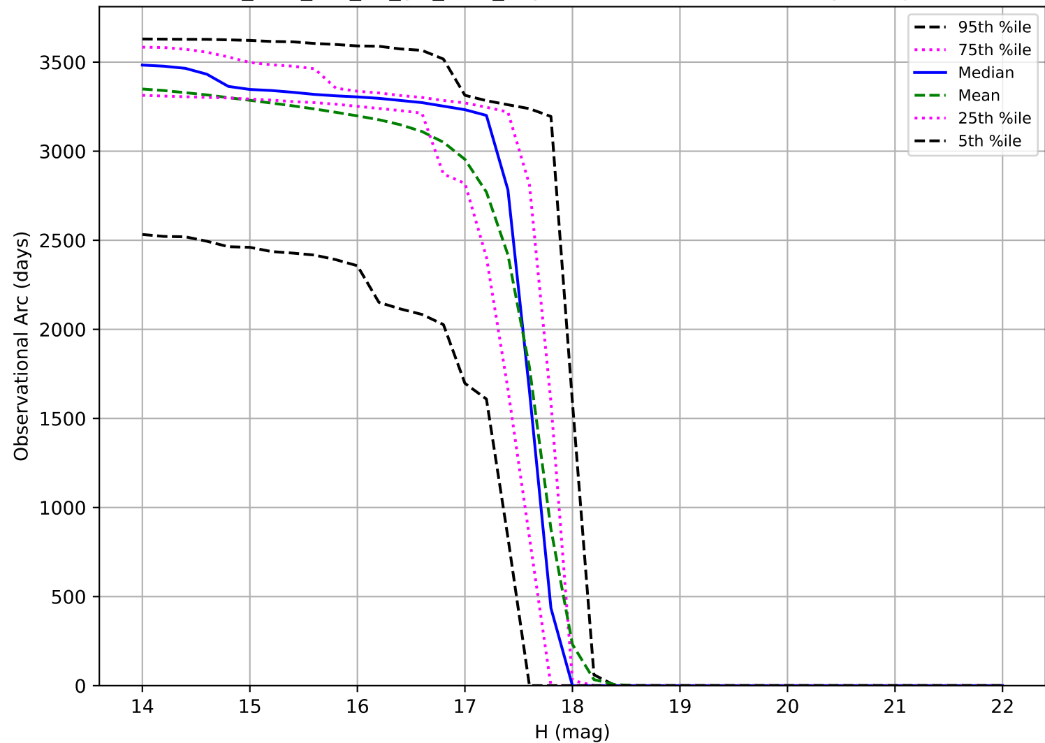
too_elab_r16_d3_giz_v3.4_10yrs: Observational Arc Length Trojan
