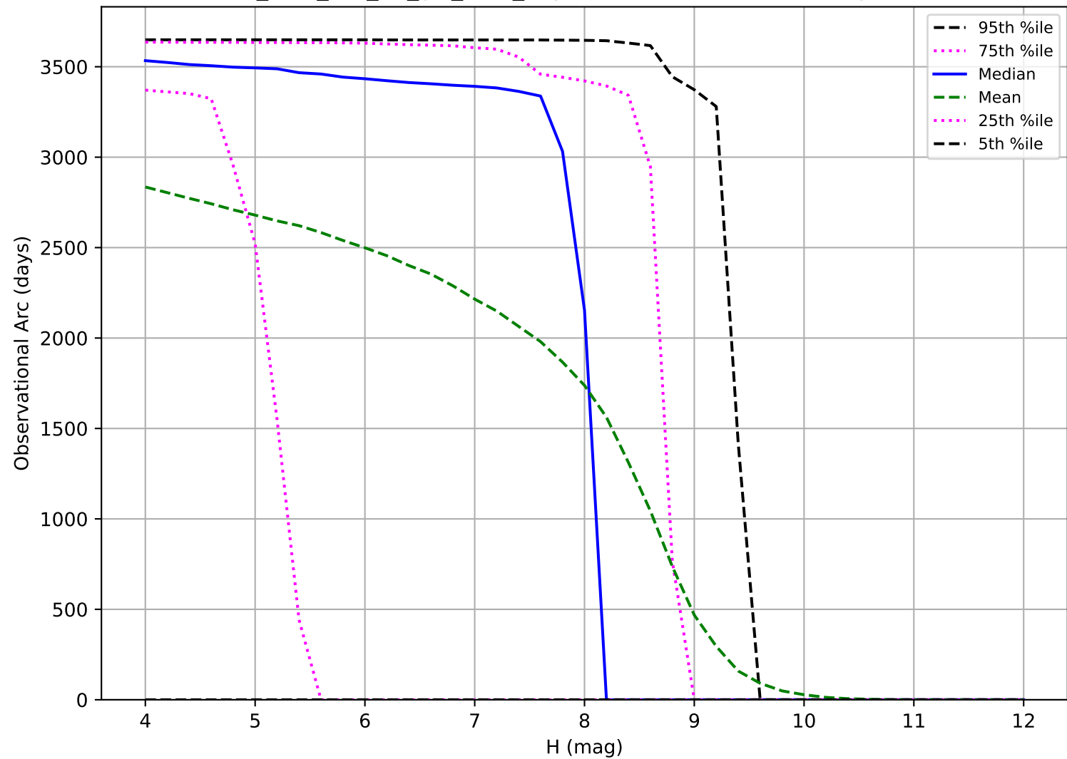
too_elab_r16_d3_giz_v3.4_10yrs: Observational Arc Length TNO
