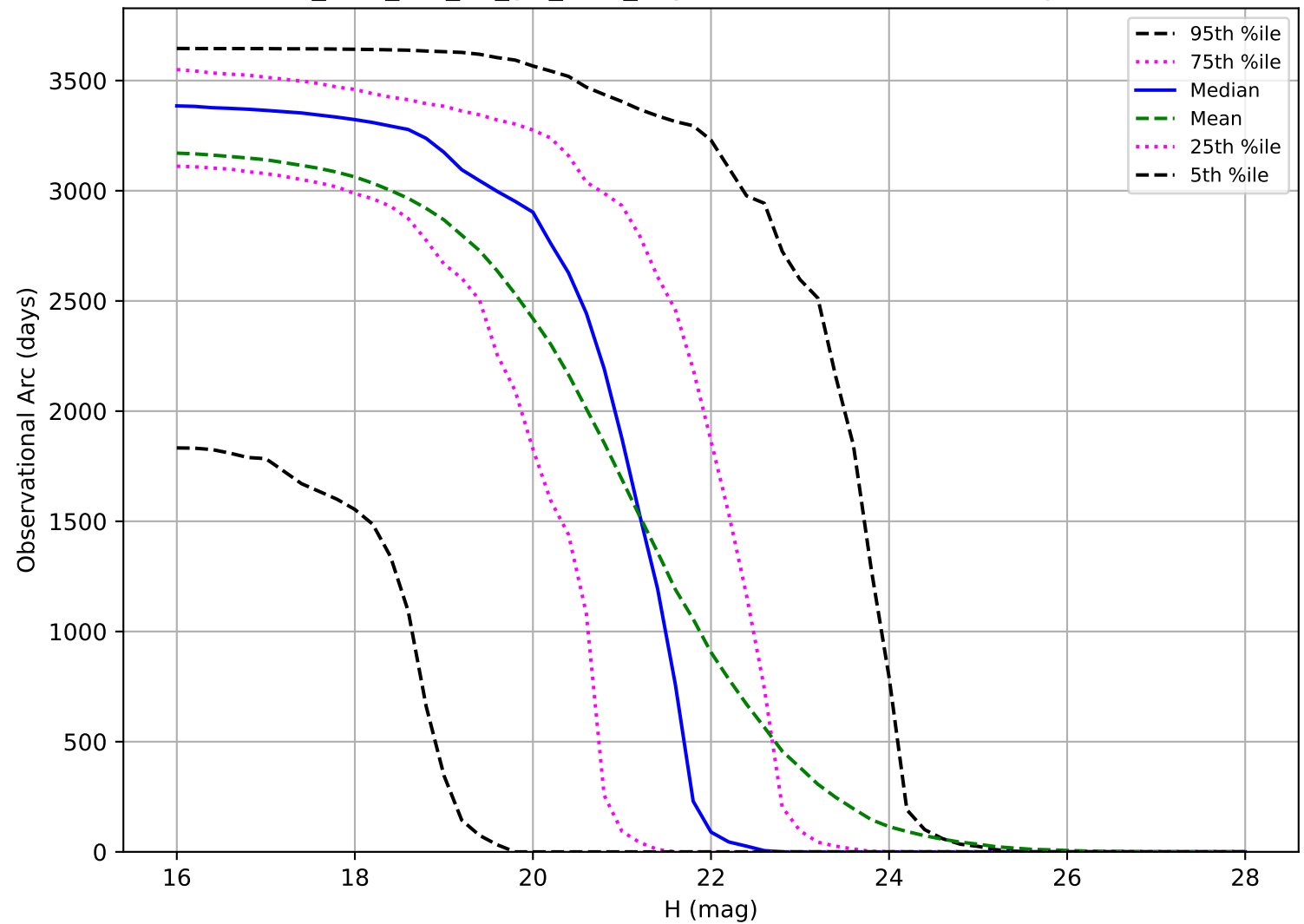
too_elab_r16_d3_giz_v3.4_10yrs: Observational Arc Length NEO
