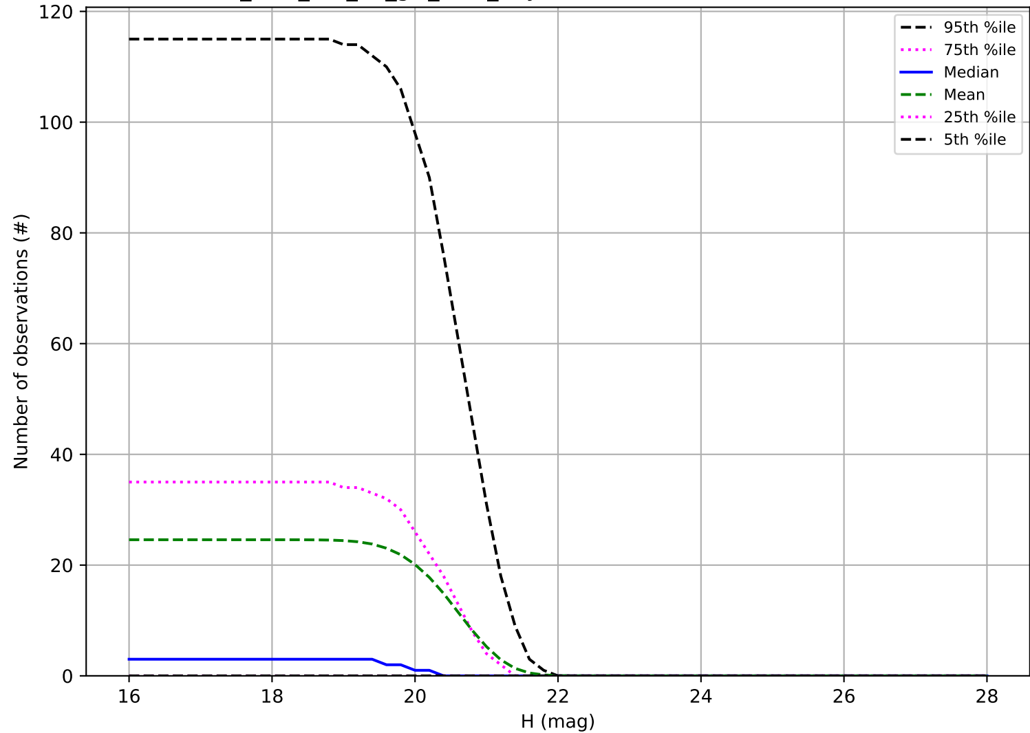
too_elab_r16_d3_giz_v3.4_10yrs: Number of observations Vatira
