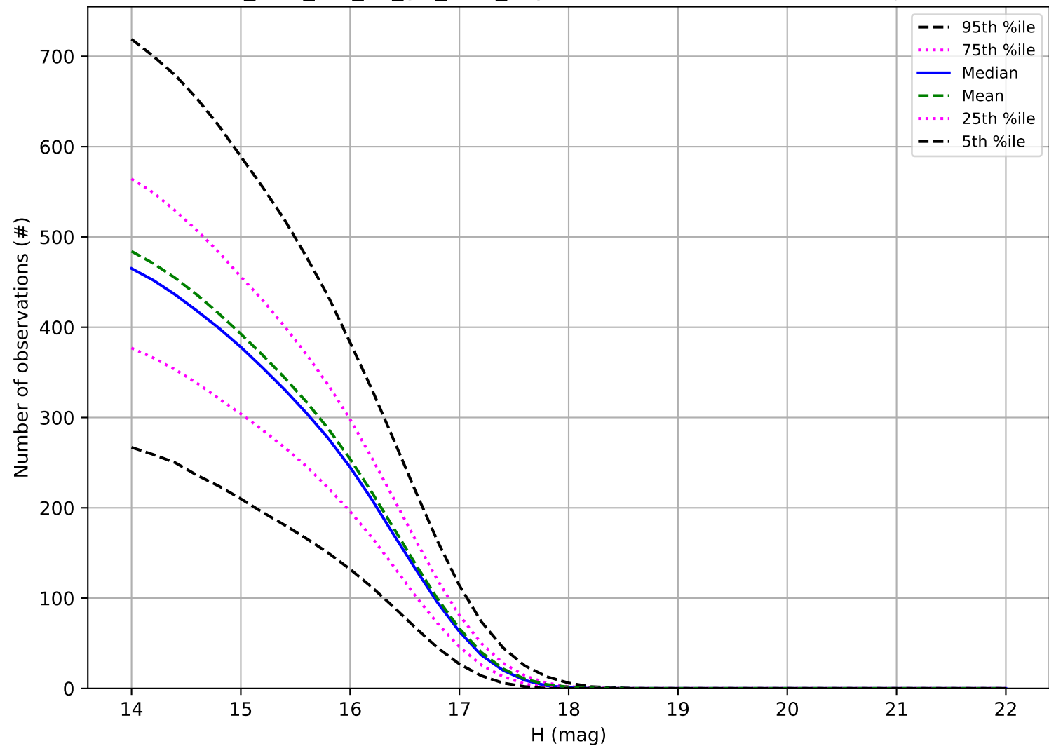
too_elab_r16_d3_giz_v3.4_10yrs: Number of observations Trojan
