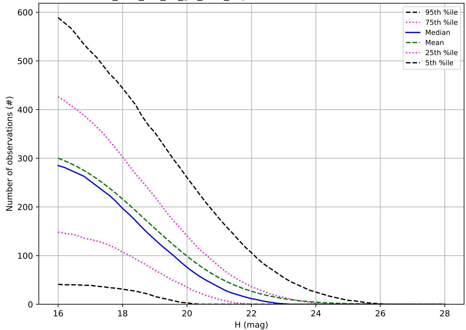
too_elab_r16_d3_giz_v3.4_10yrs: Number of observations PHA
