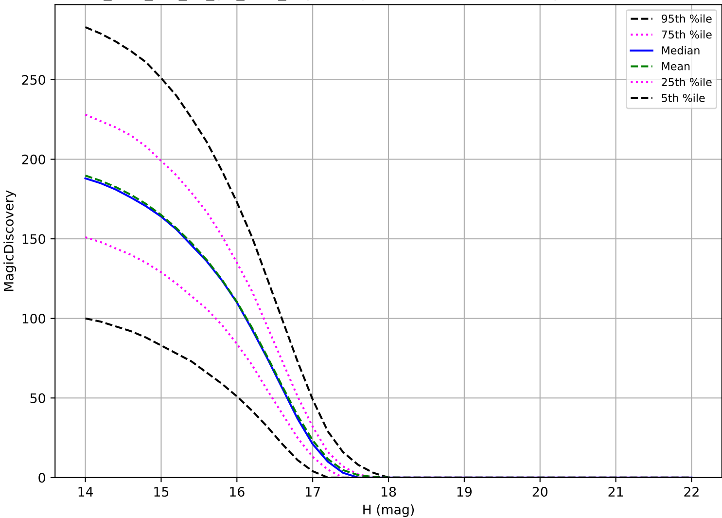
too_elab_r16_d3_giz_v3.4_10yrs: Trojan 6 detections in 60 nights detection loss
