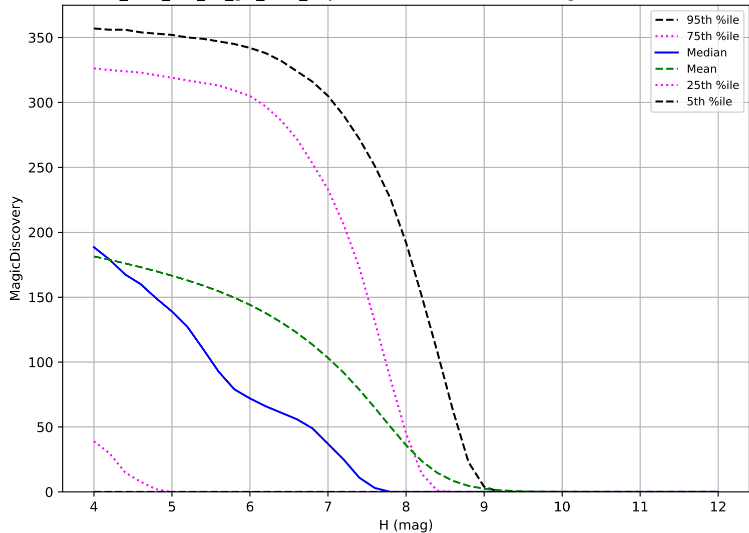
too_elab_r16_d3_giz_v3.4_10yrs: TNO 6 detections in 60 nights detection loss
