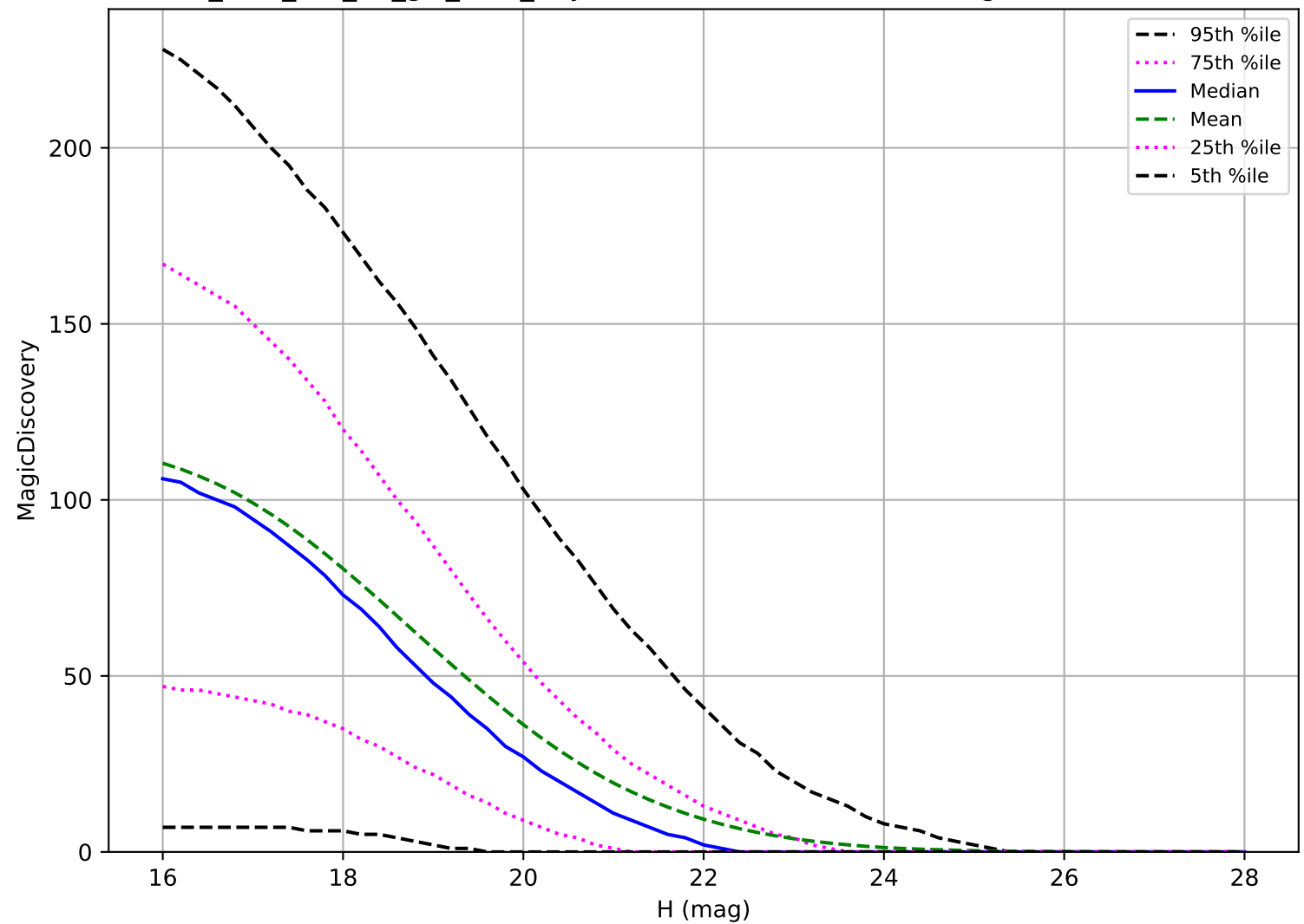
too_elab_r16_d3_giz_v3.4_10yrs: PHA 6 detections in 60 nights detection loss
