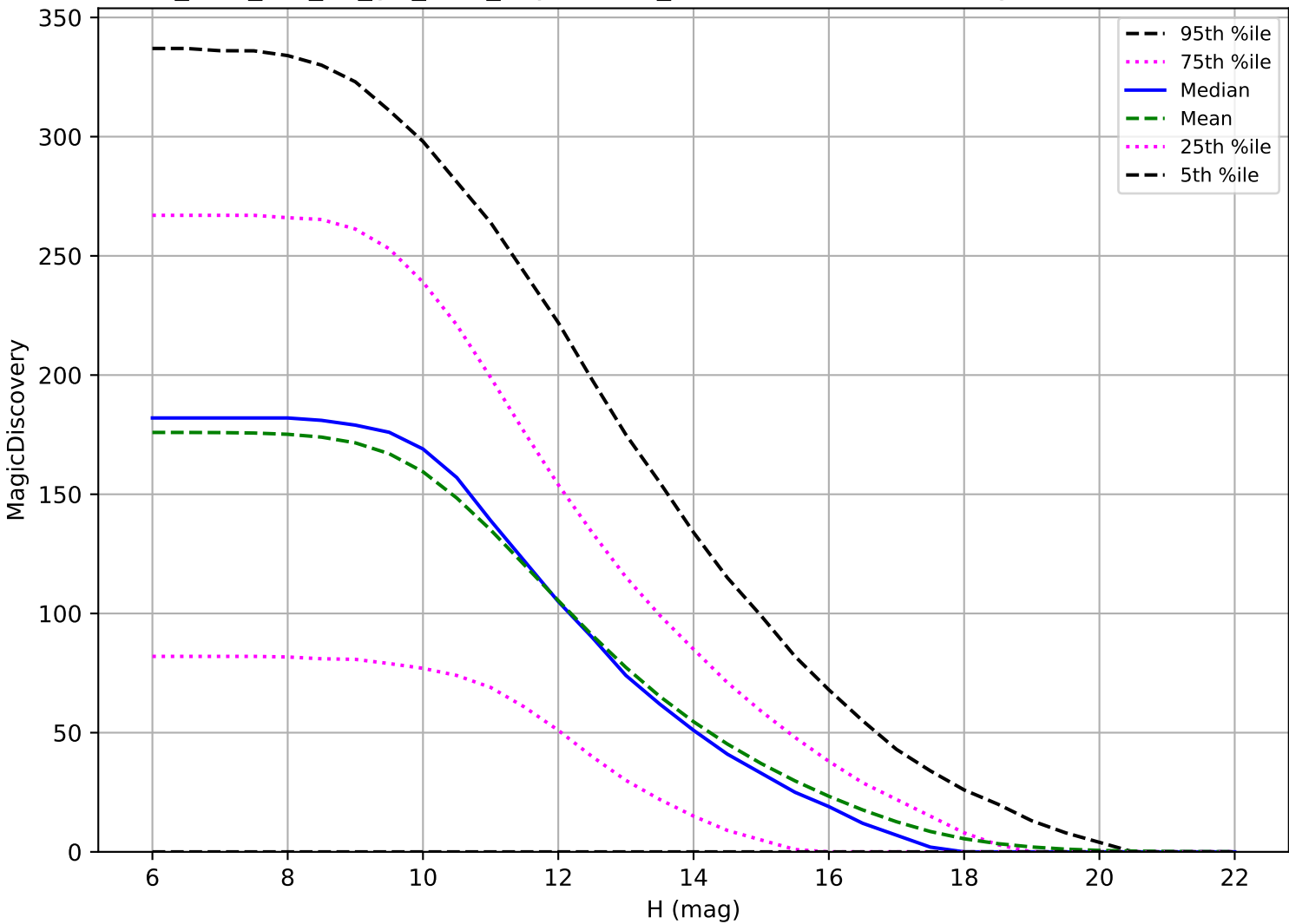
too_elab_r16_d3_giz_v3.4_10yrs: OCC_r5 6 detections in 60 nights detection loss
