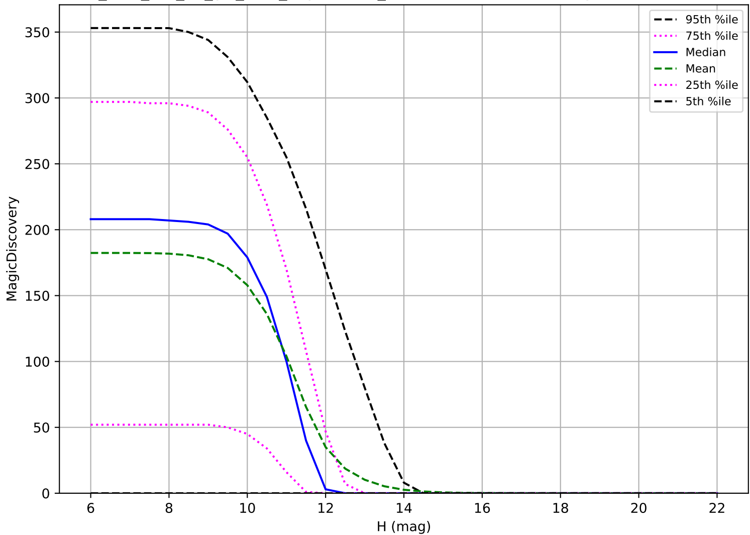
too_elab_r16_d3_giz_v3.4_10yrs: OCC_r20 6 detections in 60 nights detection loss
