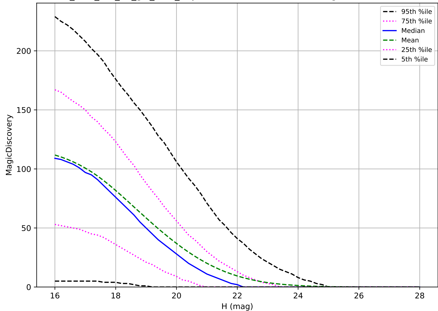
too_elab_r16_d3_giz_v3.4_10yrs: NEO 6 detections in 60 nights detection loss
