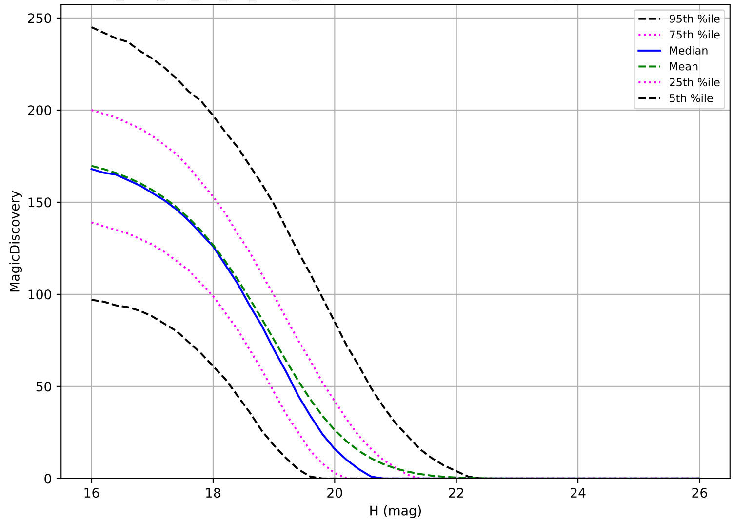
too_elab_r16_d3_giz_v3.4_10yrs: MBA 6 detections in 60 nights detection loss
