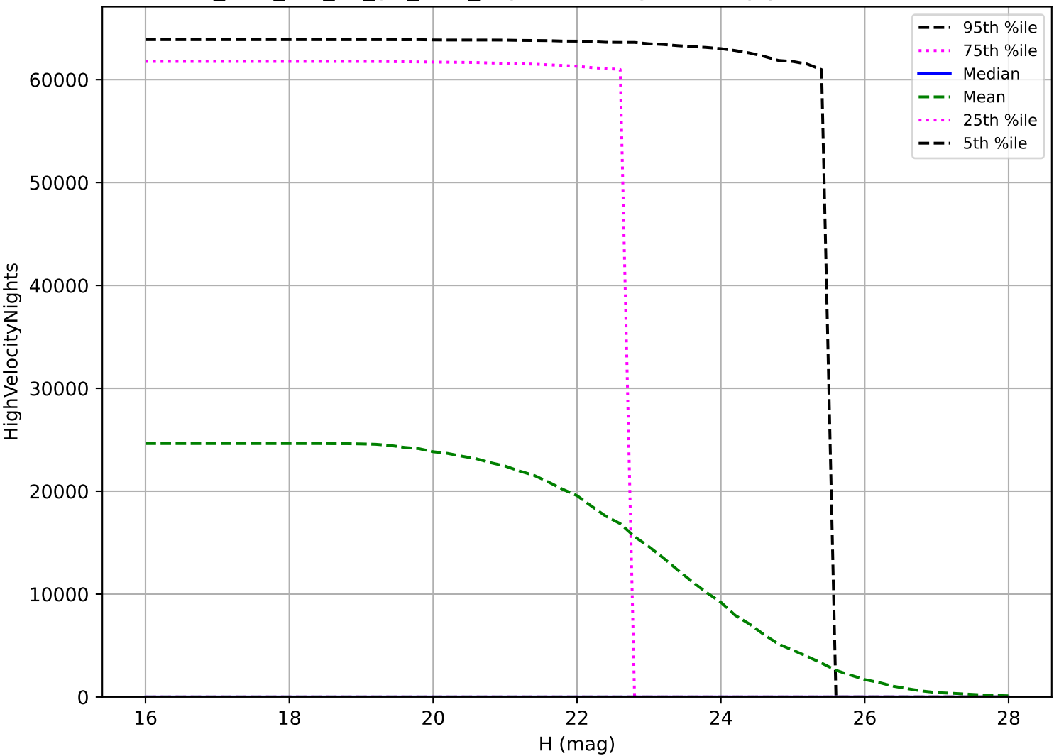
too_elab_r16_d3_giz_v3.4_10yrs: PHA High velocity pair detection loss
