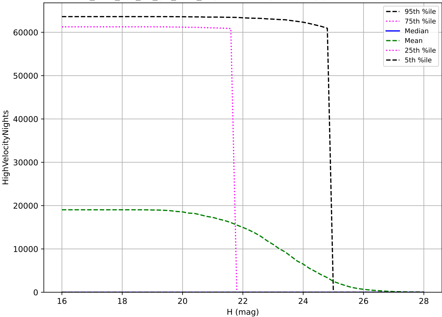
too_elab_r16_d3_giz_v3.4_10yrs: NEO High velocity pair detection loss
